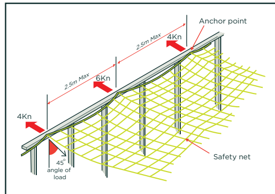
Figure 11: Attaching safety nets to timber structures.
