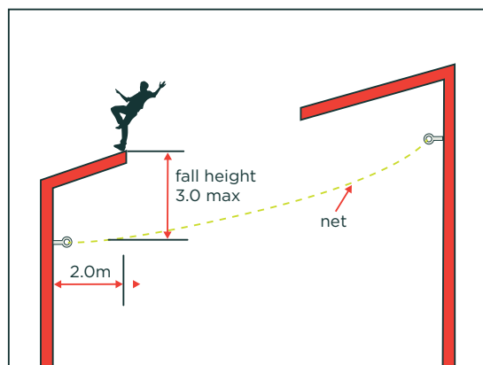
Figure 3: Fall height with 2.0 m of outer edge of net.
