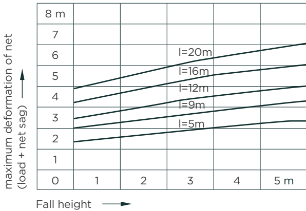
Figure 5: Deformation of net when an object falls on it.
