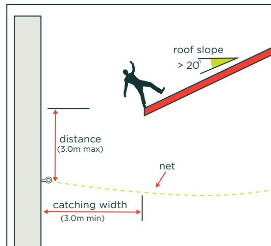
Figure 8: Fall heights where working platform has a slope of more than 20°.
