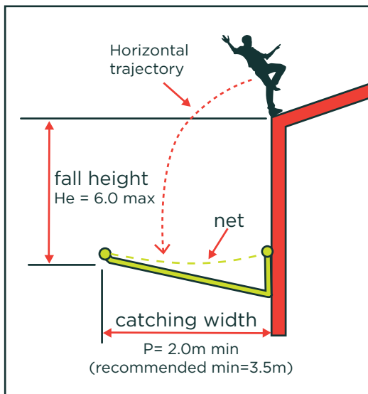
Figure 7: Catching width.
