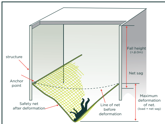
Figure 10: Minimum load-carrying capacity of anchor points.
